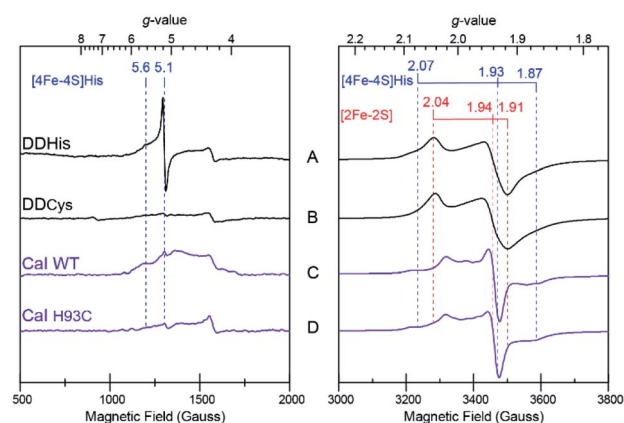
Fig. 4 X-band EPR spectra of distal domain and Cal, with low-field region on left; high-field region, on right. (A) DDHis (230 \mu M) (B) DDCys (230 \mu M) (C), Cal WT (200 \mu M) (D) Cal H93C (200 \mu M). All samples were prepared under identical conditions and reduced with dithionite in pH 8.8 buffer. Signal assignments for the [4Fe-4S]His and [2Fe-2S] clusters are indicated. Measurement conditions: microwave frequency 9.39 GHz; modulation frequency, 100 kHz; modulation amplitude, 10 Gauss; microwave power, 1 mW (A and B), 10 mW (500–2000 Gauss C and D), 1 mW (3000–4000 Gauss C and D); sample temperature: 10 K.
