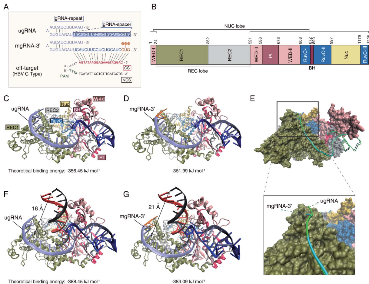
Fig. 4 Molecular docking calculations of Cas12a interacting with gRNA and off-target DNA. (A) Sequences of ugRNA , mgRNA-3' and off-target DNA for docking calculations. The gRNA-repeat sequence is marked in purple, while the gRNA-spacer is in blue. The 2'-OMe modifications of mgRNA-3' are highlighted in orange with "M". The complementary strand (CS) of off-target DNA with gRNA is shown in red, while the non-complementary strand (NCS) is shown in black. (B) The structure of the Cas12a protein. Cas12a consists of the WED-I, II, III (pink), REC1 (green) and REC2 (gray), RuvCs (dusty blue), Nuc (yellow), PI (pink brown) and BH (rufous) domains. (C) Docking result of Cas12a binding with ugRNA . The ugRNA-spacer is described in purple. (D) Docking calculations of Cas12a binding with mgRNA-3' . The 2'-OMe modifications at the 3'-end of mgRNA-3' are highlighted in orange. (E) Docking result of Cas12a interacting with ugRNA and mgRNA-3' . Top, full view. Bottom, enlarged view of the 3'-end of ugRNA and mgRNA-3' . (F) Docking result of Cas12a/ ugRNA interacting with off-target DNA. (G) Docking result of Cas12a/ mgRNA-3' interacting with off-target DNA.
