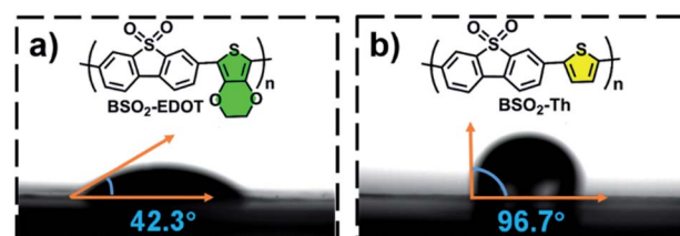
Fig. 6 Water contact angles of (a) \text{BSO}_2\text{-EDOT} and (b) \text{BSO}_2\text{-Th} .
