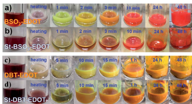
Fig. 5 Color changes of reaction mixtures with time: \text{BSO}_2\text{-EDOT} synthesized via (a) DarP and (b) Stille coupling and DBT-EDOT synthesized via (c) DarP and (d) Stille coupling.
