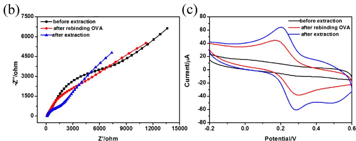
Fig. 3 (a) Schematic illustration of the synthesis of MIP-PANI particles and the fabrication of MIP-PANI sensor, (b) EIS curves and (c) CV curves of MIP-PANI particles modified electrode in [\text{Fe}(\text{CN})_6]^{3-/4-} solution before extraction, after extraction and after rebinding OVA by incubation in 0.5 \text{ mg mL}^{-1} OVA solution (reprinted with permission from Elsevier, ref. 21 Luo et al. , (2017)).
