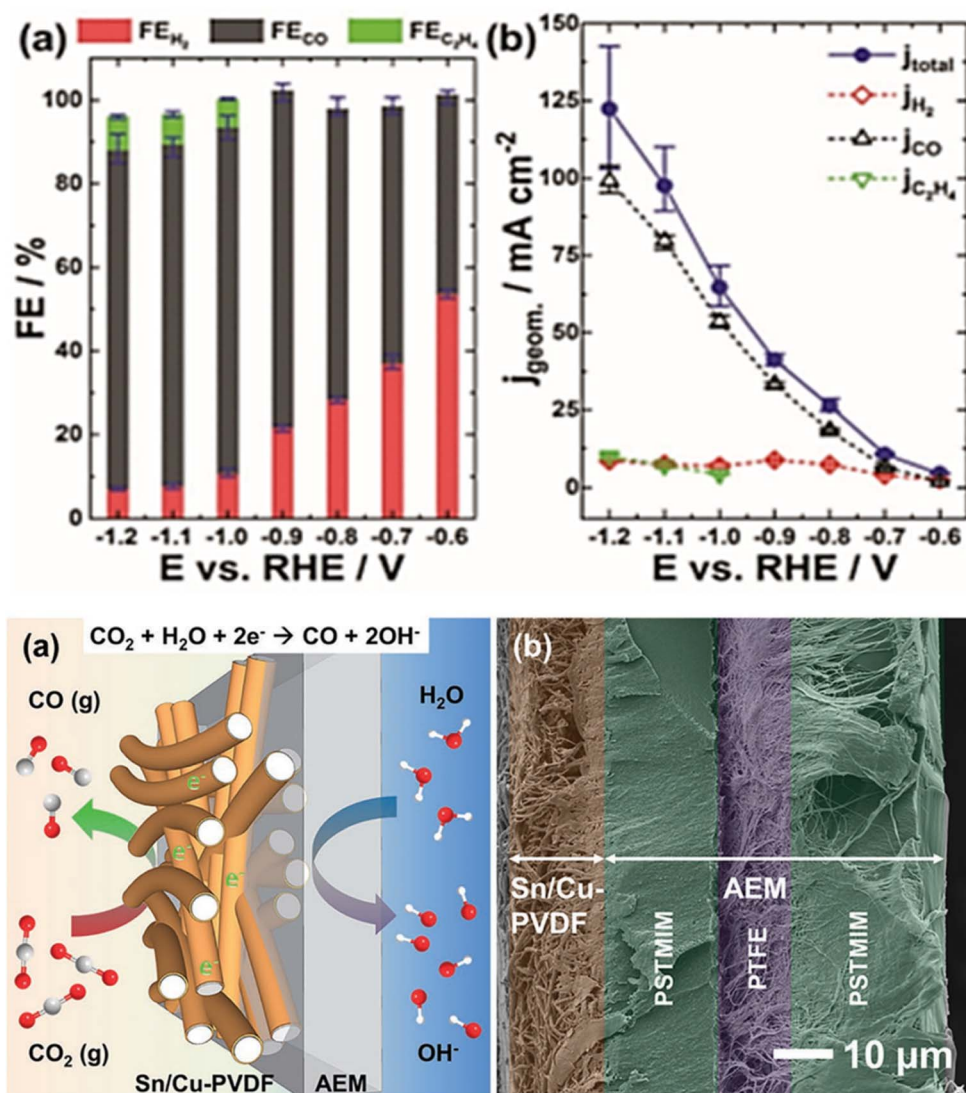
Fig. 2 (Up): (a) Faradaic efficiencies, (b) current densities for electrochemical \text{CO}_2 reduction at a Sn/Cu-PVDF GDE at ( -0.6 to -1.2 V vs. RHE). (Bottom): (a) Scheme and (b) cross-sectional SEM image of a Sn/Cu-PVDF/AEM assembly used for electrocatalytic reduction of gaseous \text{CO}_2 . Reproduced with permission. 66 Copyright ©2019, Wiley-VCH.
