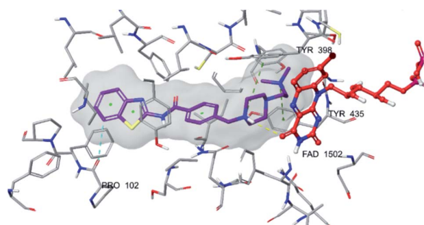
Fig. 8 3D interaction of compound 4f at binding region of MAO-B (PBDID: 2V5Z). Maroon carbons: compound 4f; red carbons: FAD protein, grey carbons: binding site residues; yellow dashes: H-bond; blue dashes: aromatic H-bond; green dashes: \pi - \pi interaction; dark green dashes: \pi -cation.
