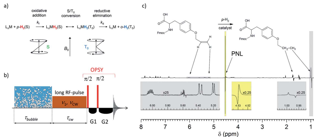
Fig. 10 (a) Magnetic conversion of p\text{-H}_2 (spin state S) to o\text{-H}_2 in spin state T_0 . (b) The PNL (Partially Negative Line) experiment for the indirect detection of the hydrogen catalyst complex. (c) ^1\text{H} NMR PHIP spectrum recorded during the hydrogenation with p\text{-H}_2 of Fmoc-O-allyl-tyrosine (left) to Fmoc-O-propyl-tyrosine (right), showing a strong PNL signal at 4.53 ppm (for details see Kiryutin et al. 93 ).
