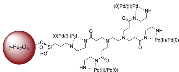
Fig. 1 The proposed structure of PAMAM G 0 -Pd@γ-Fe 2 O 3 .
