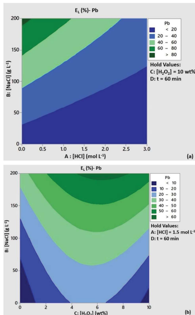
Fig. 4 Contour plots of Pb leaching efficiency as a function of (a) [HCl]/[NaCl] and (b) [H_2O_2]/[NaCl] . Conditions: L/S = 10 \text{ mL g}^{-1} , T = 80^\circ\text{C} , t = 60 \text{ min} and (a) [H_2O_2] = 10 \text{ wt\%} , (b) [HCl] = 1.5 \text{ mol L}^{-1} .
