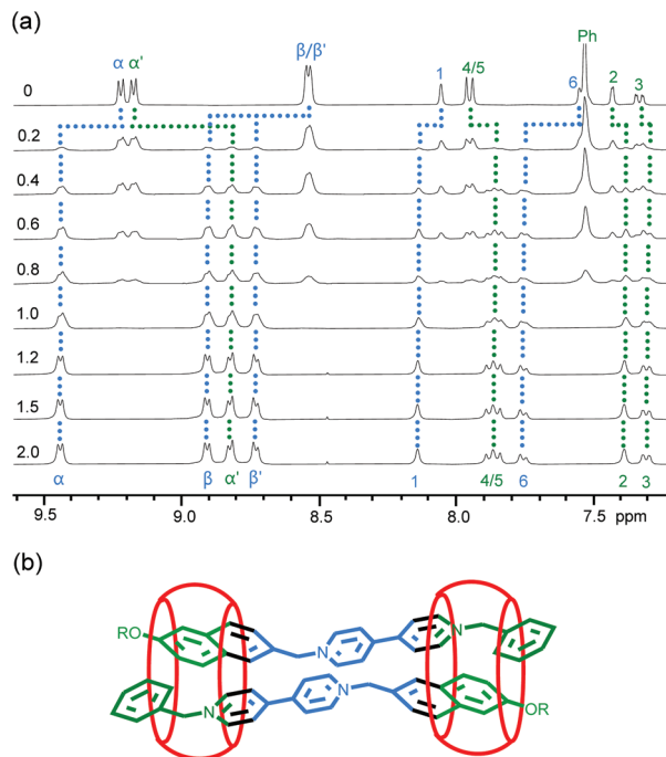
Fig. 1 (a) 1 H NMR spectra of the mixture of M1 (5.0 mM) and CB[8] (0, 0.2, 0.4, 0.6, 0.8, 1.0, 1.2, 1.5 and 2.0 equiv.) in D 2 O at 25 °C. (b) 2 + 2 binding pattern between M1 and CB[8] revealed by the above 1 H NMR spectra in D 2 O, highlighting a slipped antiparallel stacking of the aromatic units of two molecules of M1 in the cavity of the CB[8] macrocycles.
