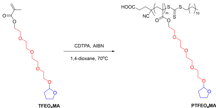
Fig. 10 Schematic depiction of the RAFT polymerization of poly(2-(2-(2-(2-(tetrahydrofuran-2-yl)oxy)ethoxy)-ethoxy)ethoxy) ethyl methacrylate) (PTFEQ 4 MA). 106
