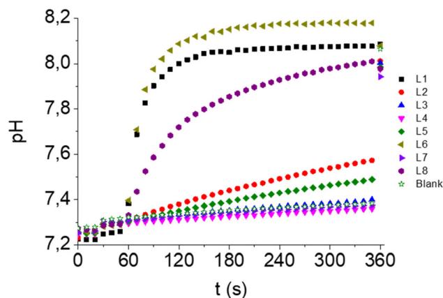
Fig. 4 Variation of pH upon addition of compounds L1 – L8 (0.5 \mu M) to 7 : 3 POPC:cholesterol vesicles (0.5 mM POPC). Vesicles (loaded with a 126.2 mM \text{NaNO}_3 solution buffered to pH 7.2 with 10 mM \text{NaH}_2\text{PO}_4 , and containing 1 mM HPTS; ionic strength (I.S.) 150 mM), were suspended in a \text{NaNO}_3 solution (126.2 mM \text{NaNO}_3 buffered to pH 7.2 with 10 mM \text{NaH}_2\text{PO}_4 ; I.S. 150 mM). At t = 30 s an aliquot of a NaOH solution (12.5 \mu L, 0.5 M) was added, and at t = 60 s the anion carrier was added. The blank is DMSO (1.25 \mu L). Each trace represents the average of at least three trials, performed with three batches of vesicles.
