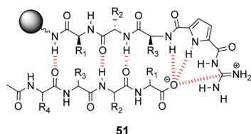
Fig. 18 GCP-based receptor library 51 generated on TentaGel®-NH 2 resin and anti-parallel \beta -sheet alignment with tetrapeptide substrates.
