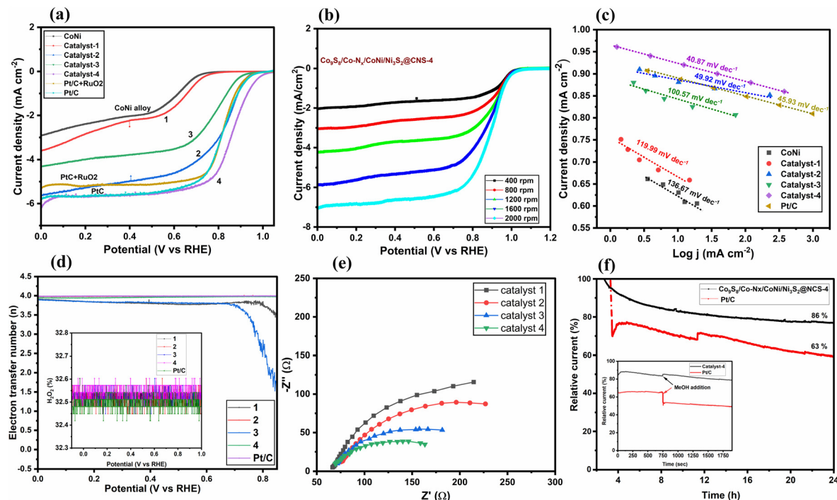
Fig. 6 Electrocatalytic ORR performances: (a) LSV curves of \text{CoS}/\text{Co-N}_x/\text{CoNi}/\text{NiS}_2@\text{CNS} 1–4, commercial 20% Pt/C and Pt/C + \text{RuO}_2 in \text{O}_2 -saturated 0.1 M KOH, (b) LSV curves of \text{CoS}/\text{Co-N}_x/\text{CoNi}/\text{NiS}_2@\text{CNS-4} , at various rotation rates, (c) Tafel plots of catalysts 1–4 and Pt/C, (d) Electron transfer number ( n ) of catalysts 1–4, and Pt/C, inset: the corresponding peroxide yields, (e) EIS spectra of catalysts 1–4, and (f) chronoamperometric responses of \text{CoS}/\text{Co-N}_x/\text{CoNi}/\text{NiS}_2@\text{CNS-4} , and commercial 20% Pt/C in \text{O}_2 -saturated 0.1 M KOH solution at a rotation rate of 1600 rpm at \sim 0.4 V vs. RHE.
