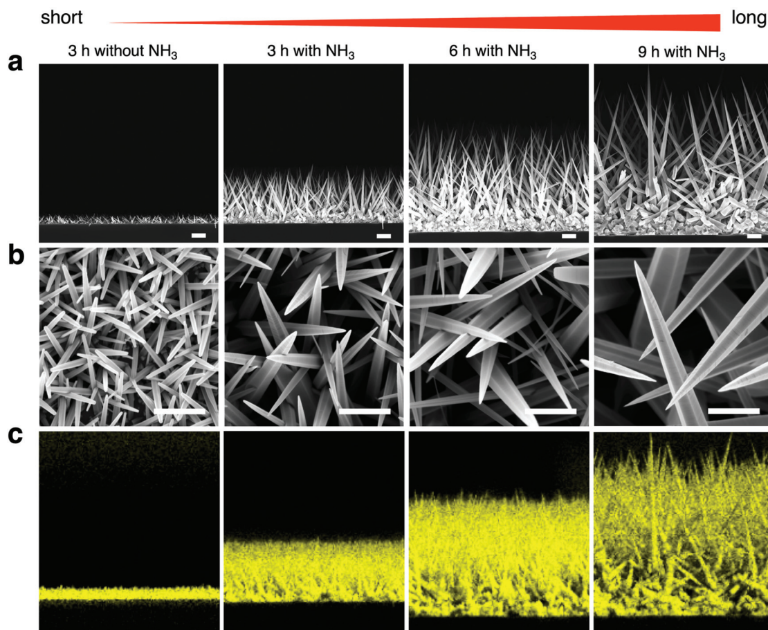
Fig. 1 (a) FESEM images of cross-sectional nanowires for different growth conditions. The scale bars are 2\ \mu\text{m} . (b) FESEM images of top-view nanowires. The scale bars are 1\ \mu\text{m} . (c) Elemental mapping of Zn K \alpha (8.6313 keV) highlighted in yellow, as a main constituent of the nanowires.
