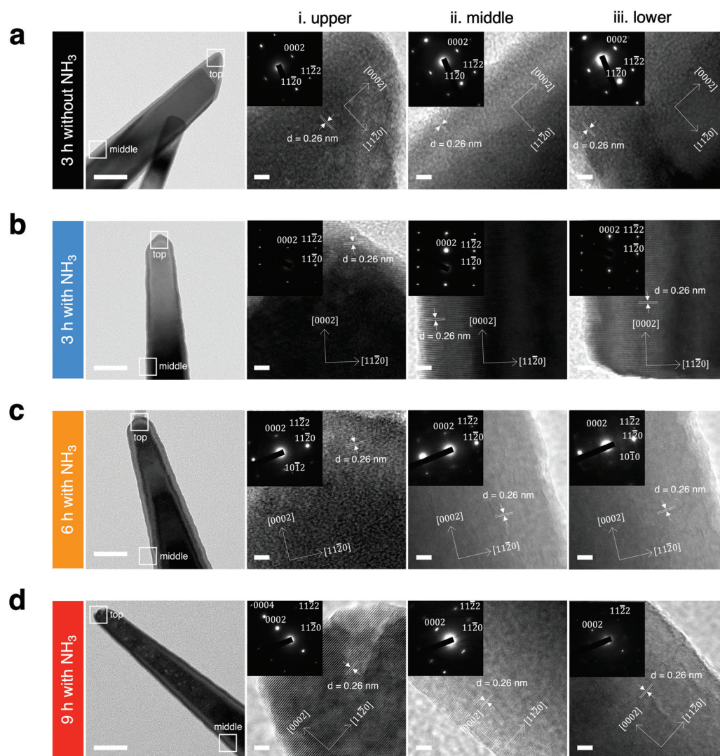
Fig. 4 (a–d) Low-resolution TEM images, and HRTEM images in three regions of i. upper, ii. middle and iii. lower of a single ZnO nanowire, where (a) is a nanowire grown for 3 h without \text{NH}_3 addition; (b) is a nanowire grown for 3 h with \text{NH}_3 addition; (c) is a nanowire grown for 6 h with \text{NH}_3 addition; and (d) is a nanowire grown for 9 h with \text{NH}_3 addition. The insets are SAED patterns of each HRTEM micrograph. The scale bars are 50 nm and 2 nm in low-resolution TEM and HRTEM images, respectively.
