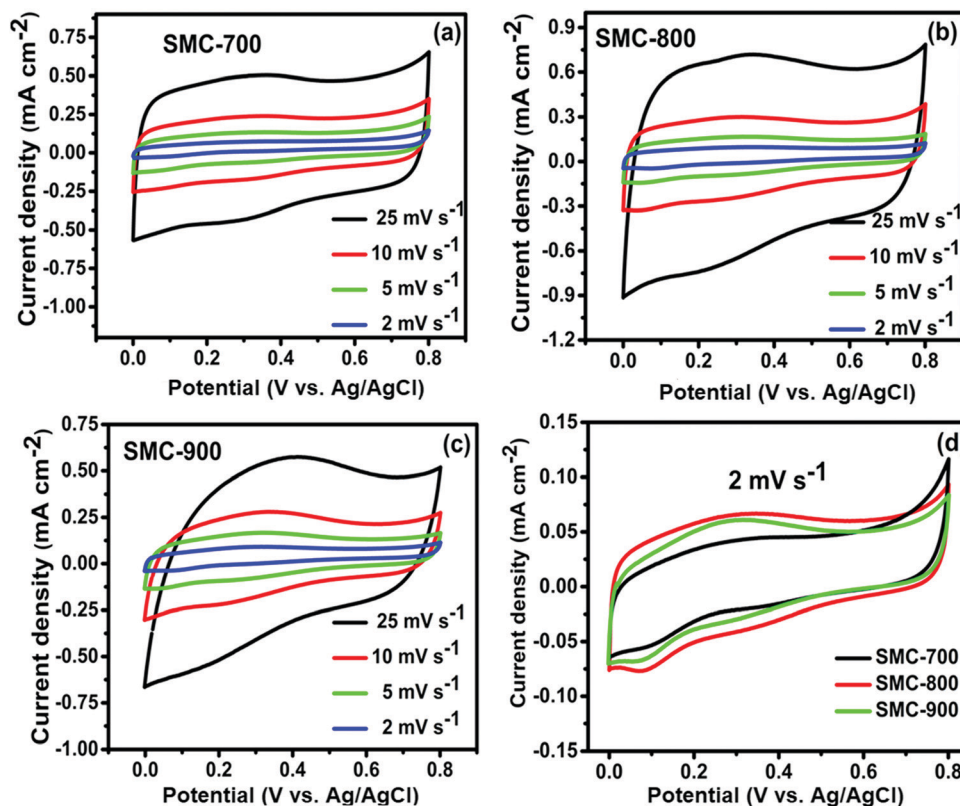
Fig. 4 (a–c) CV curves at different scan rates for SMC-700, 800, and 900, and (d) CV curves at a scan rate of 2 \text{ mV s}^{-1} .
