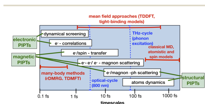
Fig. 3 Timescales of elementary excitations and decay processes in complex quantum materials. The blue dashed lines indicate the time-period of single-cycle of optical pulse and THz electric field which excites electrons and phonons, respectively. This figure has been adapted/reproduced from ref. 45 and 46 with permissions from Elsevier and John Wiley and Sons, copyrights 1997 and 2012.
