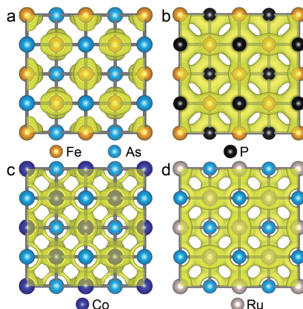
Fig. 4 Isosurface plots of the partial charge density of state 1 in FeAs (a), FeP (b), CoAs (c) and RuAs (d) monolayers with an isosurface value of 0.054 \text{ e}^{-3} .
