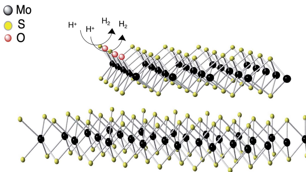
Fig. 7 Schematic representation of HER mechanism of conductive MoS 2 . Hydrogen evolution reaction process at the edges of conductive MoS 2 .
