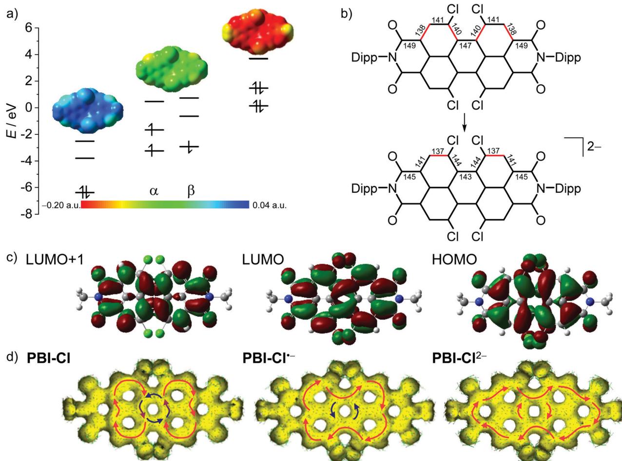
Fig. 4 (a) The HOMO, LUMO and LUMO+1 levels as obtained from DFT calculations of PBI-Cl (left), the corresponding \alpha - and \beta -spin MO levels of PBI-Cl •- (middle) and HOMO-1, HOMO and LUMO levels of PBI-Cl 2- (right), as well as the electrostatic potential maps of the respective derivative (top, isovalue 0.020 a.u.). (b) Calculated bond length for perylene carbon-carbon bonds in neutral and dianionic states in pm (for details, see Table S4, ESI†). Bonds drawn in red indicate a high double-bond character. (c) The HOMO, LUMO and LUMO+1 (right to left) of PBI-Cl . The corresponding orbitals of PBI-Cl •- and PBI-Cl 2- are visually indistinguishable. Orbitals and electrostatic potential maps were calculated using DFT (B3LYP/6-31g(d)). (d) Calculated AICD isosurface plots of PBI-Cl , PBI-Cl •- and PBI-Cl 2- . Clockwise ring current is depicted with red arrows and counterclockwise ring current with blue arrows (isosurface value 0.025).
