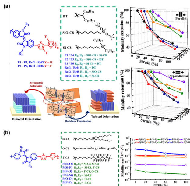
Fig. 9 Tuning the electrical-mechanical properties of conjugated polymers via asymmetric side-chain engineering. (a) Asymmetrical side-chain engineering of IIT-based polymers structure; illustration of the effects of the asymmetric side-chain design and backbone fluorination on chain packing; and the mobility retention of these polymers with different strains and with the stretching force parallel and perpendicular to the charge-transporting direction. 122 Copyright: 2019, the American Chemical Society. (b) Structure of isoindigo-bithiophene (IIT)-based conjugated polymers with three types of side chains and the orthogonal hole mobilities values of the stretched polymer films with strain ranging from 0 to 100%. 123 Copyright: 2021, the American Chemical Society.
