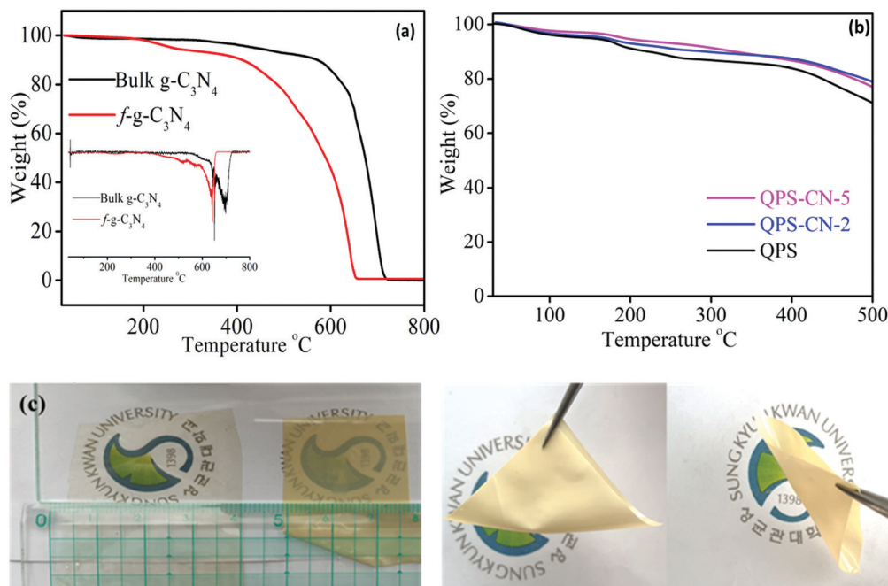
Fig. 5 TGA behavior of the (a) bulk and functionalized g-C_3N_4 (dTg spectra inserted) and (b) QPS and QPS-CN _x membranes. (c) Optical images of the QPS and QPS-CN-5 membranes.
