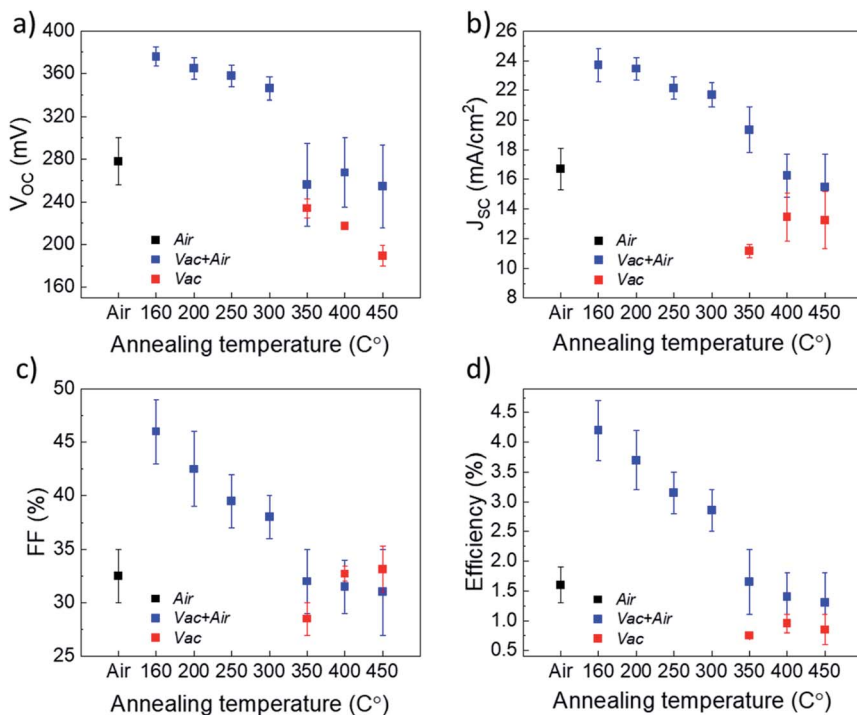
Fig. 3 J–V parameters, including (a) open-circuit voltage – V_{OC} , (b) short-circuit current density – J_{SC} , (c) fill factor – FF and (d) efficiency of \text{TiO}_2/\text{Sb}_2\text{Se}_3 devices with different \text{TiO}_2 annealing conditions.
