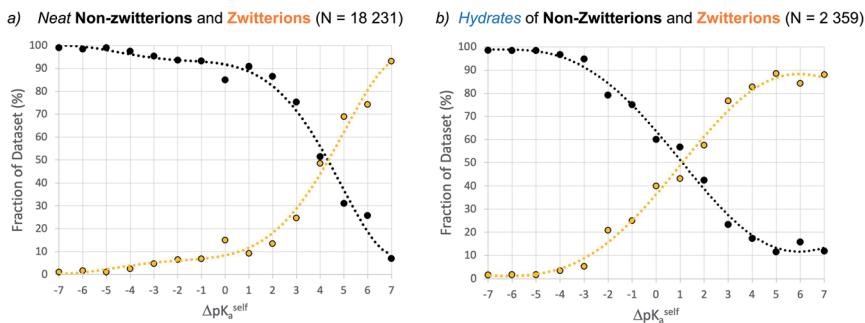
Fig. 9 Relative occurrence (%) of non-zwitterions (black) versus zwitterions (orange) as a function of \Delta pK_{a, self} (bins of one \Delta pK_a unit). Data for unsolvated forms (a) are compared to hydrates (b). Dataset-2 is filtered according to: only one main component, no Q4 zwitterions.
