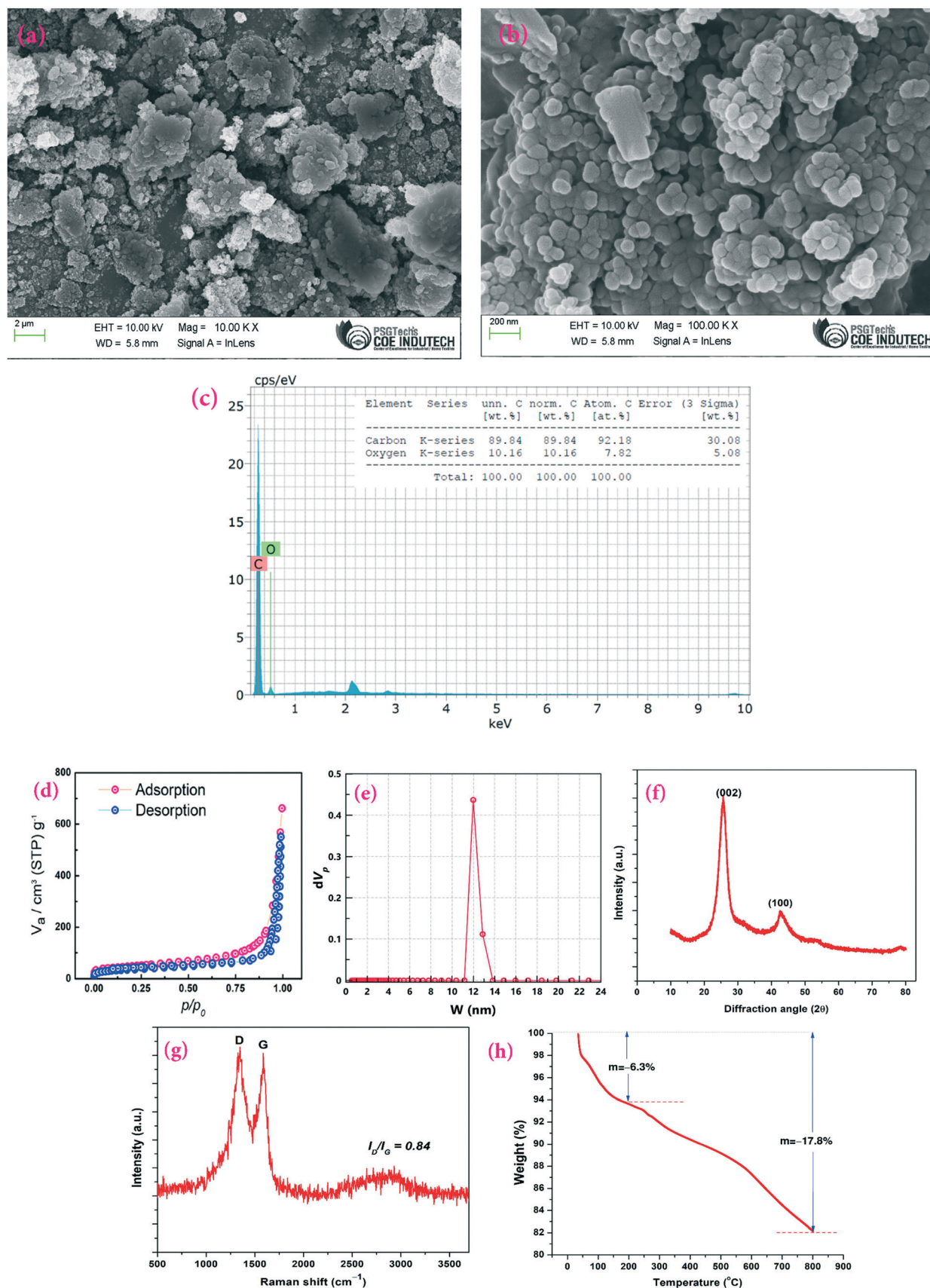
Fig. 3 Characterization of the produced CSCNP using SEM micrographs at magnifications of (a) 2 μm and (b) 200 nm; (c) EDX analysis showing the percentage of the elements present; (d) N 2 adsorption/desorption isotherm; (e) NLDFT/GCMC pore size distribution analysis; (f) XRD diffractogram; (g) Raman spectrum; and (h) thermogravimetric analysis.
