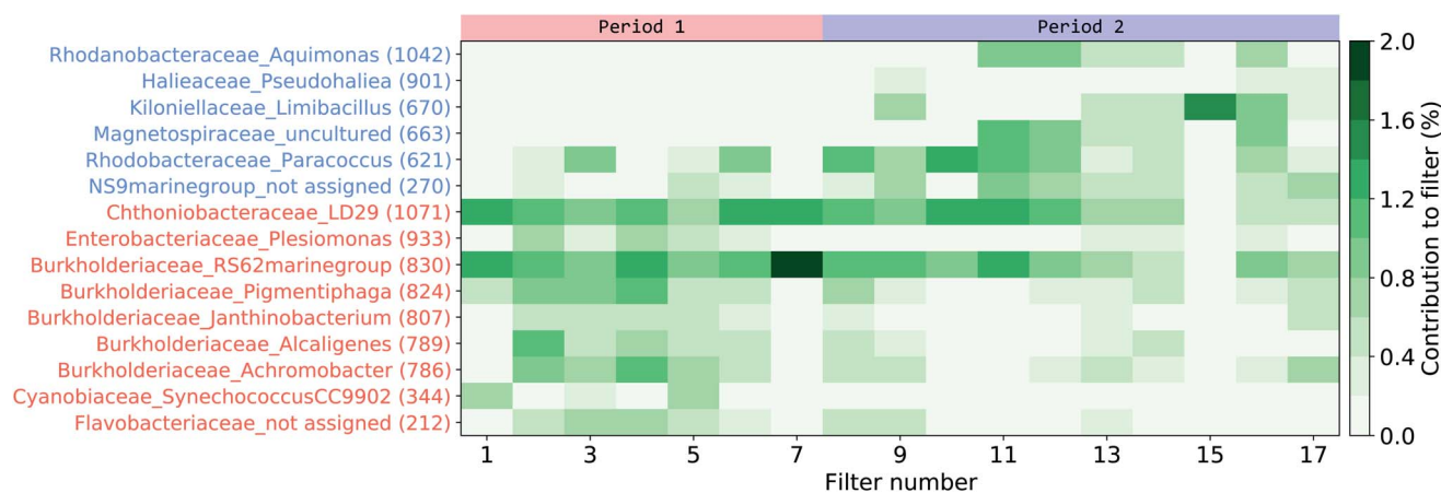
Fig. 7 Indicator organism (IO) analysis of the aerosol filter samples. Organisms pointed out by the LEfSe analysis as characterizing either the first (red indicator organism (IO) numbers) or the second period (blue IO numbers) have their contribution per filter signal shown. For full taxonomy classification refer to Table S3† in the ESI.
