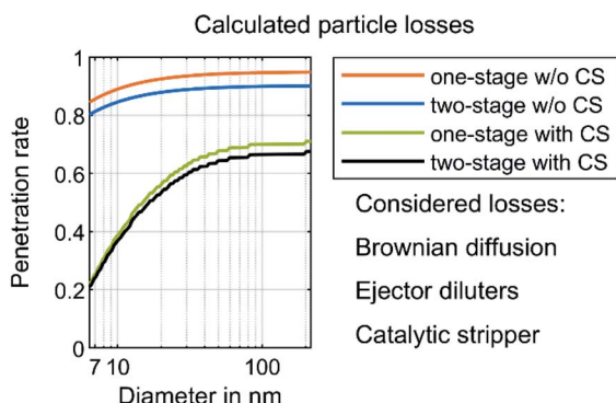
Fig. 2 Calculated particle losses. The losses due to Brownian diffusion are based on calculations according to Hinds 54 with the assumption of a laminar flow inside the tubing. The losses of each ejector diluter were assumed to be 5% according to Giechaskiel et al. 60 The manufacturer of the catalytic stripper determined the respective penetration efficiency at a nominal flow rate of 10 \text{ l min}^{-1} .
