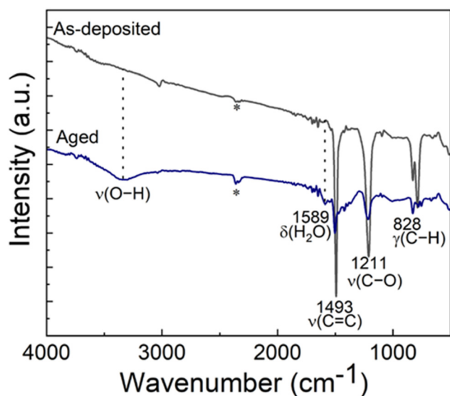
Fig. 6 Stability studies of the Zn-HQ thin films deposited at 60 °C on Si(100) in this study. Comparison of FTIR spectrum of a 95 nm thick Zn-HQ thin film immediately after the deposition and after two weeks in ambient conditions. The bands marked with * are caused by adsorbed \text{CO}_2 .
