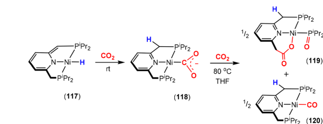
Scheme 36 Reactivity of nickel–hydride pincer type complexes with \text{CO}_2 and subsequent transformation.
