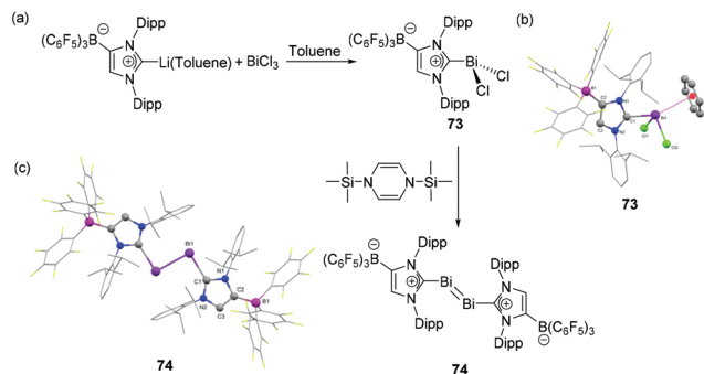
Fig. 24 (a) Syntheses of NHC-stabilized bismuth adduct 73 , and dibismuthene compound 74 ; solid-state structures of 73 (b) and 74 (c).
