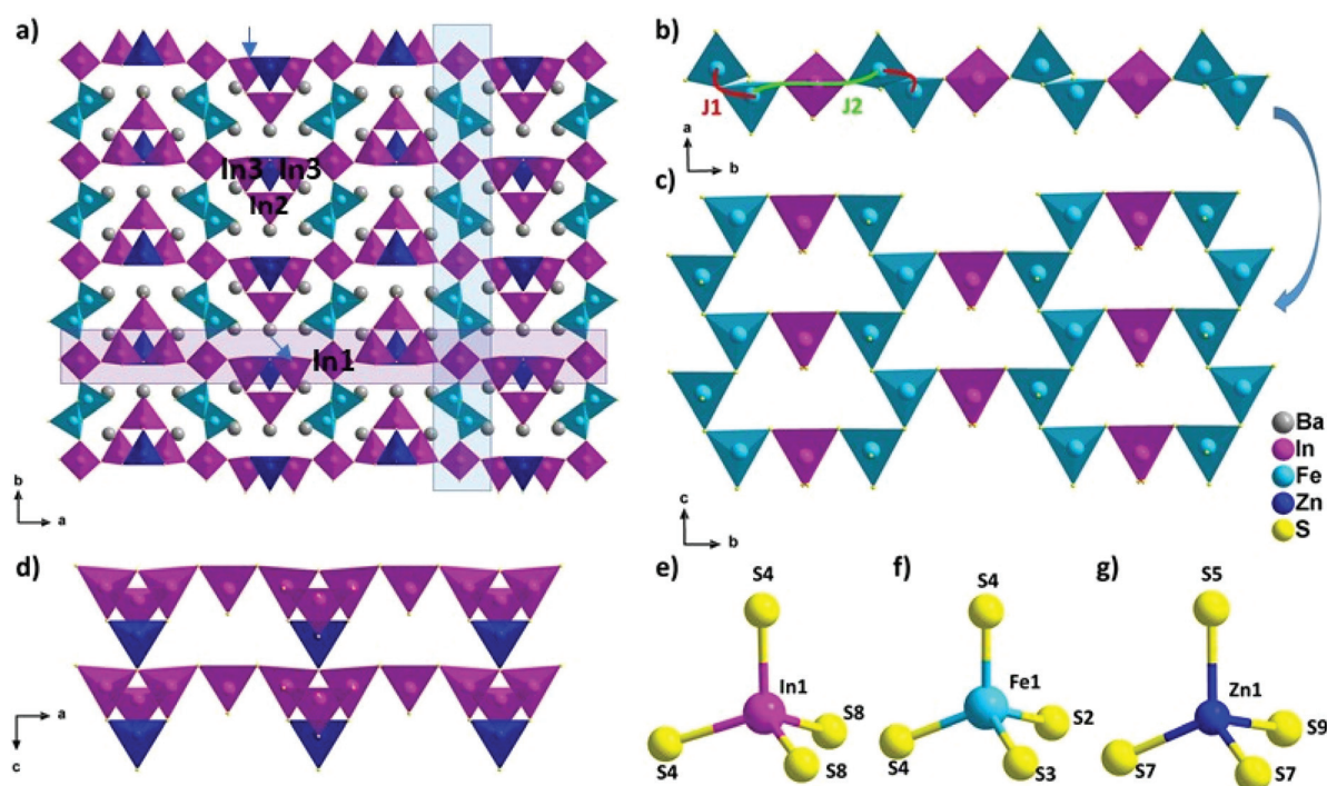
Fig. 1 (a) View of Ba 5 Fe 2 ZnIn 4 S 15 along the c axis, (b) magnetic exchange coupling J1 and J2 in the chains extended along the b axis, (c) interconnection between magnetic chains, (d) view of lined chains of type 2, and (e–g) In1, Fe1 and Zn1 coordination, respectively.
