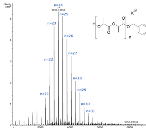
Fig. 4 MALDI-ToF-MS spectrum of PLA synthesized by 1 ([LA]/[ 1 ] = 20, T = 80\text{ }^{\circ}\text{C} ).
