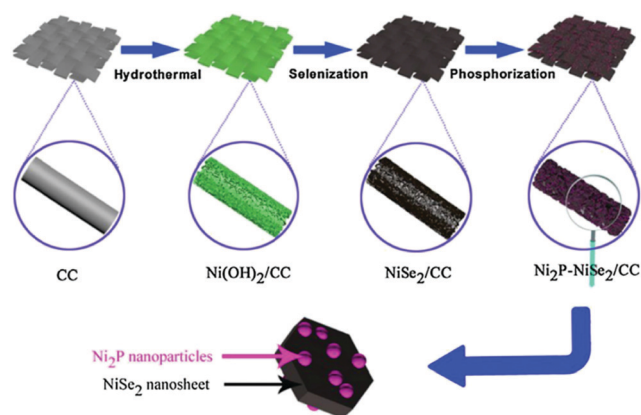
Fig. 81 Schematic illustration of synthesis of \text{Ni}_2\text{P} - \text{NiSe}_2/\text{CC} hetero-structure catalyst. Reproduced with permission from ref. 1188 Copyright Elsevier 2020.
