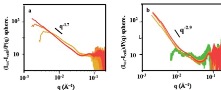
Fig. 10 Structure factor, S(q) , of the nanocrystals embedded in cells incubated with nanocrystals (a) and supraballs (b) at the different time points ( 30 \text{ min} (green), 4 \text{ hours} (yellow), 1 \text{ day} (orange) and 2 \text{ days} (red)).
