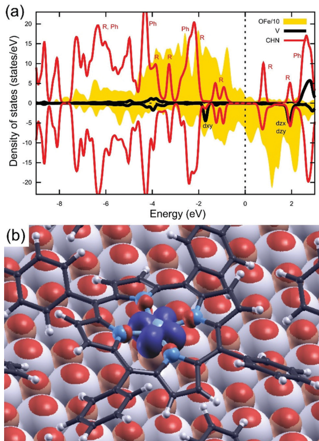
Fig. 7 (a) Projected density of states (DOS) of adsorbed VOTPP in the Odwn@Fe configuration (spin minority contributions are shown with negative sign). (b) Spin polarization of the system (difference between the spin-majority and spin-minority electron densities). The isovalue shown is \pm 0.02 \text{ \AA}^{-3} .
