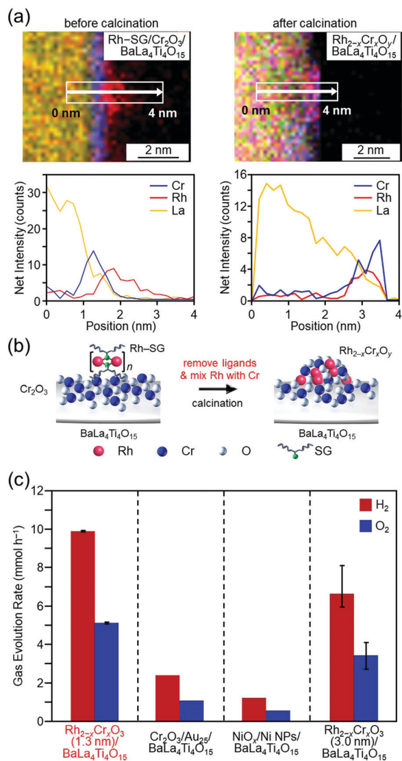
Fig. 16 HAADF-STEM images of Rh-SG complexes adsorbed on the Cr 2 O 3 /BaLa 4 Ti 4 O 15 photocatalyst before and after calcination (Rh-SG/Cr 2 O 3 /BaLa 4 Ti 4 O 15 and Rh 2-x Cr x O 3 /BaLa 4 Ti 4 O 15 , respectively). (a) Line analysis of elemental mapping of Rh-SG/Cr 2 O 3 /BaLa 4 Ti 4 O 15 (left) and Rh 2-x Cr x O 3 /BaLa 4 Ti 4 O 15 (right). (b) Schematic of the phenomenon that occurred during the calcination process. (c) Comparison of the gas-evolution rates over different photocatalysts: Rh 2-x Cr x O 3 (1.3 nm)/BaLa 4 Ti 4 O 15 (0.09 wt% Rh and 0.10 wt% Cr), Cr 2 O 3 /Au 25 /BaLa 4 Ti 4 O 15 (0.10 wt% Au and 0.50 wt% Cr), Ni NiO x /NPs/BaLa 4 Ti 4 O 15 (0.50 wt% Ni), and Rh 2-x Cr x O 3 (3.0 nm)/BaLa 4 Ti 4 O 15 (0.10 wt% Rh and 0.15 wt% Cr). Reproduced with permission from ref. 290. Copyright 2020 Wiley-VCH.
