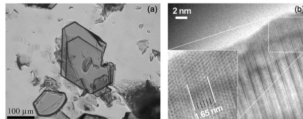
Fig. 10 (a) Optical image of single crystals of \text{InFeO}_3(\text{ZnO})_4 . (b) HRTEM images of \text{InFeO}_3(\text{ZnO})_4 imaged along \langle 2\bar{1}\bar{1}0 \rangle zone axis. Dark spot lines have the In-layer spacing of 1.65 nm. Panels (a and b) are reprinted with permission from ref. 54. © 2014 John Wiley and Sons, Inc.
