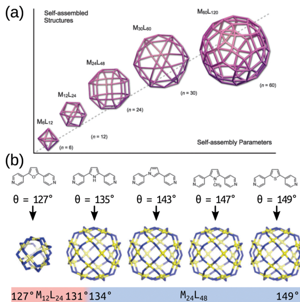
Fig. 2 (a) A schematic of the structure relationships observed in a family of roughly spherical coordination polyhedra with general formula M_nL_{2n} , where metals ( M ) and bridging bis(pyridine) ligands ( L ) are mapped onto the respective vertices and edges of the polyhedra. (b) Critical structural switch between Pd_{12}L_{24} and Pd_{24}L_{48} structures in a chemically well-defined system as a function of ligand bite angle. Reprinted with permission from ref. 40.
