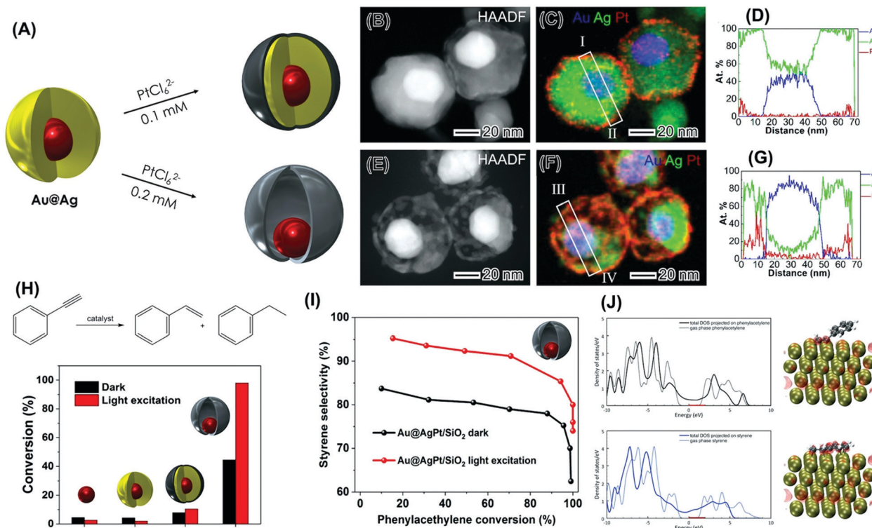
Fig. 9 (A) Synthesis of plasmonic-catalytic Au@AgPt core-shell (top) and Au@AgPt nanorattles (bottom) via the galvanic replacement reaction between \text{PtCl}_6^{2-}(\text{aq}) and Ag in Au@Ag core-shell NPs. 100 (B–G) STEM analysis for Au@AgPt core-shell (B–D) and Au@AgPt nanorattles (E–G). 100 (B and E) HAADF image in which the brightest contrast from Au core results from its higher Z (atomic number) as Z_{\text{Au}} > Z_{\text{Pt}} > Z_{\text{Ag}} . (C and F) Corresponding composite elemental map EDS elemental maps of Au (blue), Ag (green), and Pt (red). (D and G) Atomic-percent distribution from quantified EDS line scan along the line I–II (D) marked in (C) and along line III–IV (G) marked in (F). (H) Scheme for the phenylacetylene hydrogenation reaction leading to the formation of styrene and ethylbenzene and conversion (%) in the dark and under visible light excitation (black and red bars, respectively) employing supported Au, Au@Ag, Au@AgPt core-shell NPs, and Au@AgPt nanorattles as catalysts. (I) Styrene selectivity as a function of conversion percentages for Au@AgPt nanorattles under dark (black trace) and visible light excitation conditions (red trace). 100 (J) DFT-calculated projected density of states of phenylacetylene (top panel) and styrene (bottom panel) in the gas phase (dotted trace) and adsorbed on Pt (solid trace). The optimized structure and integrated state from the Fermi Level (0 eV) to 2 eV are also shown. 100 Reprinted (adapted) with permission from ref. 100. Copyright 2018 American Chemical Society.
