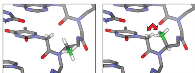
Fig. 5 A model of the \beta PNA structure showing a different degree of steric clash between the \beta -(S)- or \beta -(R)-methyl groups and the nucleobase side arm (reprinted from ref. 36, Copyright (2011), with permission from Elsevier).
