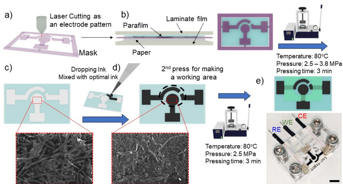
Fig. 1 Schematic diagram of the fabrication process with parafilm hot pressing for an electrochemical paper-based device with a three carbon-electrode system. (a) The patterning mask was cut with laser cutting. (b) Parafilm, patterning mask, and CHR paper were orderly stacked to create hydrophobic/hydrophilic patterns. (c) Parafilm was melted and pressed through a patterned laminate mask for making hydrophobic (blue colour) and hydrophilic (white colour) areas. (d) Optimal carbon conductive ink was added onto the hydrophilic area to create the carbon electrodes (counter, working and reference). The pores of the paper matrix are filled with the ink as shown in SEM images. (e) Subsequently, the working area was defined by additional parafilm pressing. The PCEs were inserted into custom-made connectors to support the connection of working, reference, and counter electrodes with the potentiostat to perform the electrochemical assay. The scale bar represents 1 cm.
