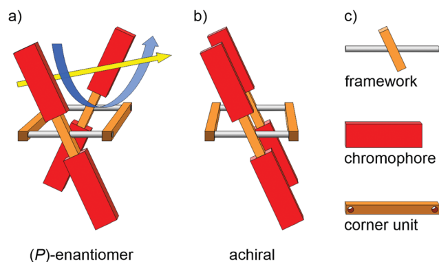
Fig. 1 Concept to fix the spatial arrangement of four chromophores by a tight rectangular scaffold. (a) The (P)-enantiomer is depicted to display the helical chirality emerging from the fixed chromophores. The yellow arrow is the view direction helping to spot the helically arranged chromophores (visualized by the blue arrow). (b) Illustration of the achiral configuration with parallel arranged chromophores. (c) Legend explaining the various subunits of the scaffold.
