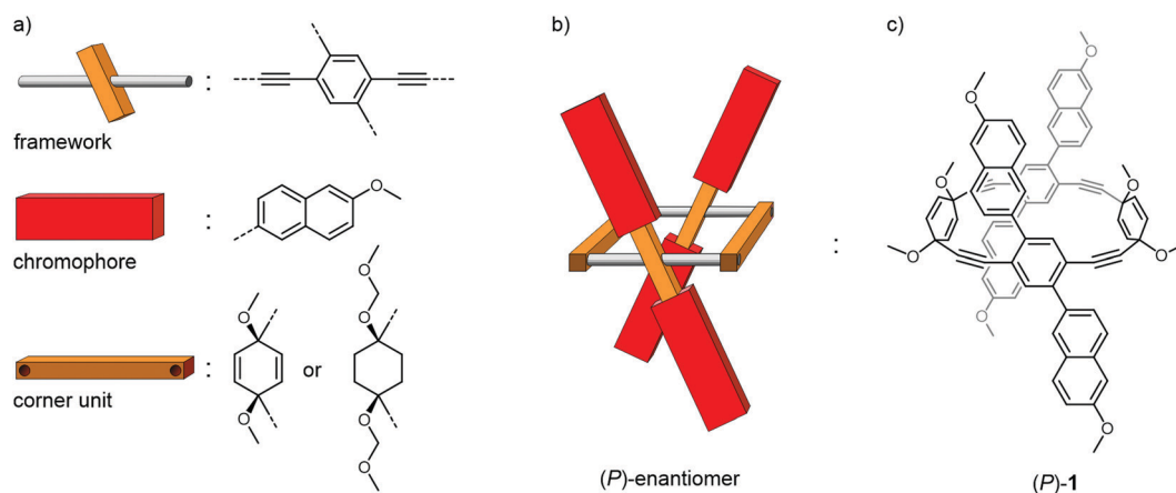
Fig. 2 (a) The molecular subunits representing the functional building blocks. (b) Conceptual picture of the (P)-enantiomer and (c) its realization with the molecular subunits using 1,4-cyclohexadiene corner units resulting in the target structure (P)-1.
