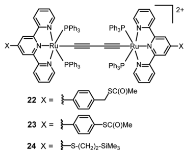
Fig. 10 Structures of 22–24.
