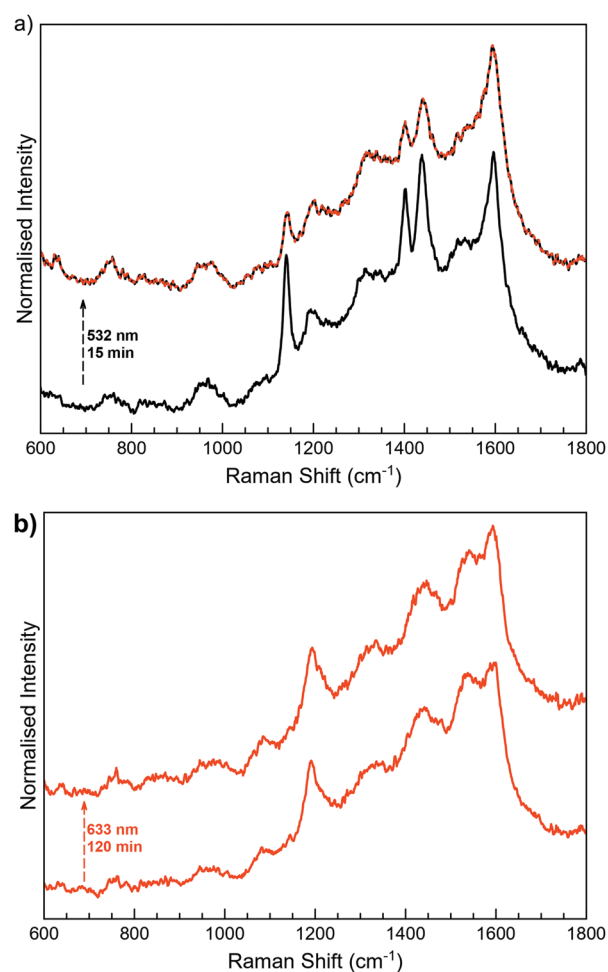
Fig. 7 Raman spectra of the irradiated \text{MoS}_2\text{-3o} (a) and \text{MoS}_2\text{-3c} (b) samples deposited on \text{SiO}_2 (285 nm)/Si substrates measured with a 532 nm excitation laser with 1% laser power. The open- and the closed-ring isomers and a mixture of both of them are represented by black, red and black-red lines, respectively. The spectra were normalised for comparison purposes.
