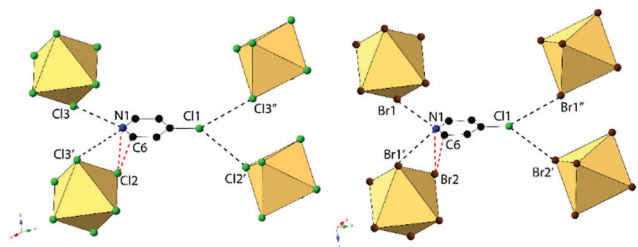
Fig. 4 Local structure of isomorphous compounds 2 (left) and 6 (right) showing halogen and hydrogen bonding (black) between [TeX_6]^{2-} octahedra and the halogen substituent on the pyridinium. Also shown is the short X \cdots N/C contacts between the protonated nitrogen N1 and carbon C6 and the metal bound halide Cl2 (red).
