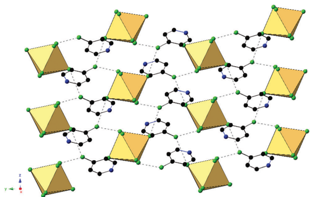
Fig. 5 Packing of 2 highlighting the extended halogen bonding (dashed lines) between [TeCl_6]^{2-} octahedra and associated ClPy cations.
