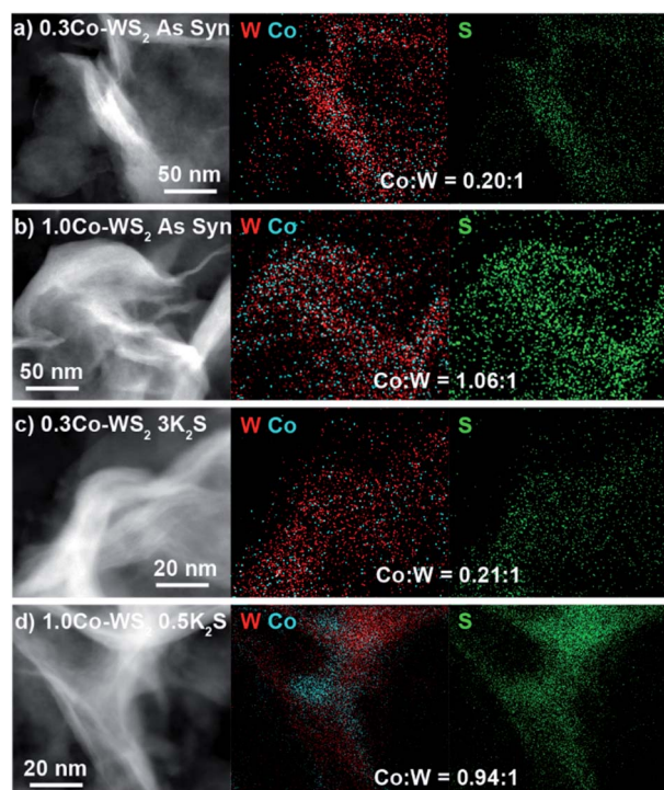
Fig. 2 STEM-EDS image and elemental maps of W, Co, and S for (a and b) as-synthesized 0.3Co and 1.0Co-WS 2 supported on C as well as (c and d) 0.3Co and 1.0Co-WS 2 after annealing with K 2 S.
