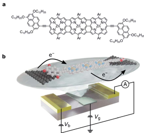
Fig. 1 (a) The molecular structure of FP3 : the edge-fused porphyrin trimer core is functionalized in the terminal meso positions by trido-decyloxyphenyl groups for anchoring to graphene source and drain electrodes. Ar groups are solubilizing aryl groups, 3,5-bis(trihexylsilyl) phenyl. (b) Device architecture: nanometer-separated graphene source and drain electrodes are electroburnt from a graphene ribbon between two gold electrodes. The graphene is patterned into a bowtie shape, and a local gate electrode separated from the molecule by a thin layer of \text{HfO}_2 (grey) is used to shift the molecular energy levels. For clarity, the bulky side-groups are omitted.
