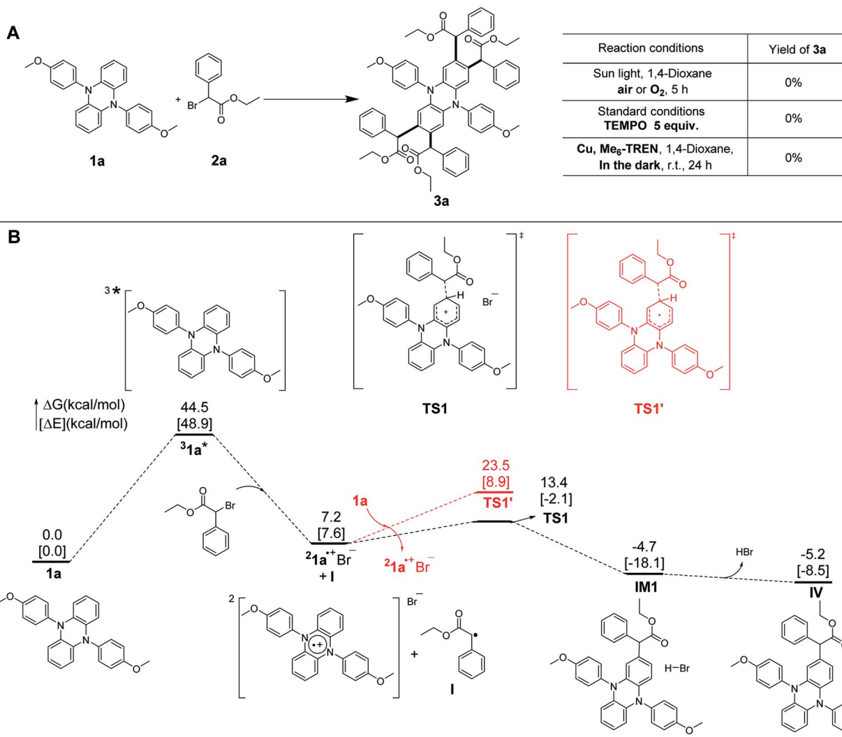
Fig. 4 Mechanistic investigations. (A) Control experiments. (B) Computed Gibbs energy profile ( \Delta G in kcal mol -1 ) and electronic energy [ \Delta E in brackets] at the BP86+D3(BJ)/def2-TZVPP (CPCM, SOL = DMAC)//BP86+D3(BJ)/def2-SVP (CPCM, SOL = DMAC) of the reaction. The proposed mechanism is simplified as a monosubstituted core modification of 1a .
