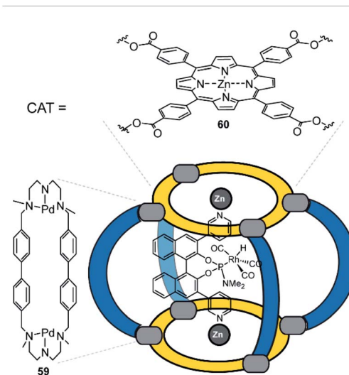
Fig. 29 A heteroleptic coordination cage that contains a hydroformylation catalyst. The assembly drives transformation of styrene selectively to the branched product with an ee of 74%. Reproduced from ref. 137 with permission from the Royal Society of Chemistry, copyright 2021.
