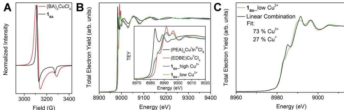
Fig. 3 (A) EPR spectra of 1_{\text{BA}} (black) and (\text{BA})_2\text{CuCl}_4 (red). (B) XAS spectra of (\text{PEA})_4\text{CuIn}^{\text{III}}\text{Cl}_8 (black), (\text{EDBE})\text{Cu}^{\text{II}}\text{Cl}_4 (red), and 1_{\text{BA}} prepared using high (blue) and low (green) solution concentrations of \text{Cu}^{2+} ( \text{EDBE} = 2,2'-(\text{ethylenedioxy})\text{bis}(\text{ethylammonium}) ). (C) A linear combination of the (\text{PEA})_4\text{CuIn}^{\text{III}}\text{Cl}_8 and (\text{EDBE})\text{Cu}^{\text{II}}\text{Cl}_4 XAS spectra (black) provides an approximation to the XAS spectrum of 1_{\text{BA}} prepared using a low solution concentration of \text{Cu}^{2+} (green), giving a rough estimate of the \text{Cu}^{2+} : \text{Cu}^+ ratio (73 : 27) for this sample (see Section 2.3.3 for a more accurate value).
